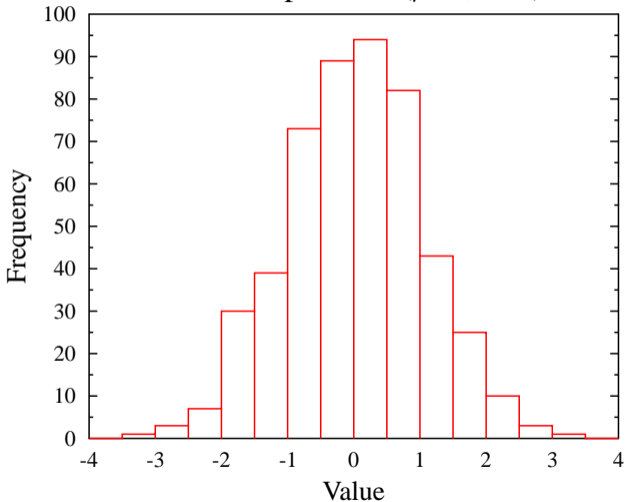
1000 samples of N(\mu=0, \sigma=1)
