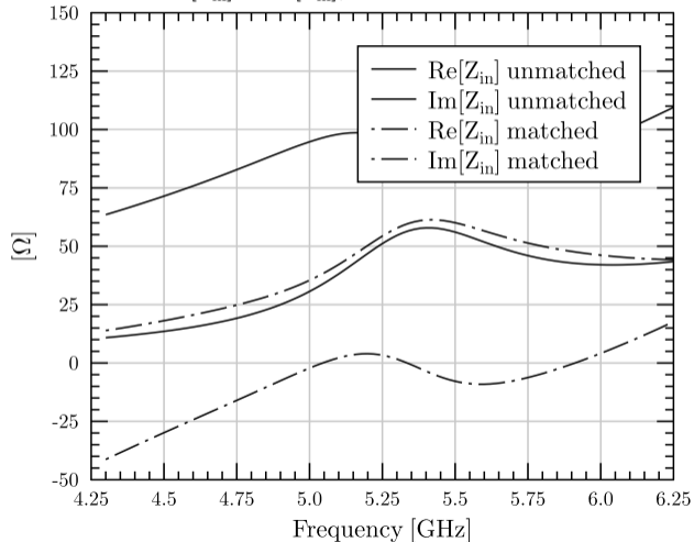
\text{Re}[Z_{\text{in}}] & \text{Im}[Z_{\text{in}}] , matched vs. unmatched
