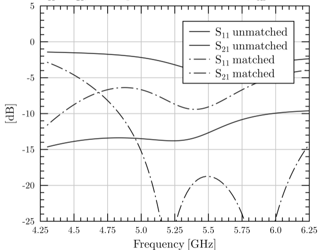
S_{11} & S_{21} , 20 mm patch on 4 mm RH31HF, f_{\text{ofs}}=7.5\text{mm}
